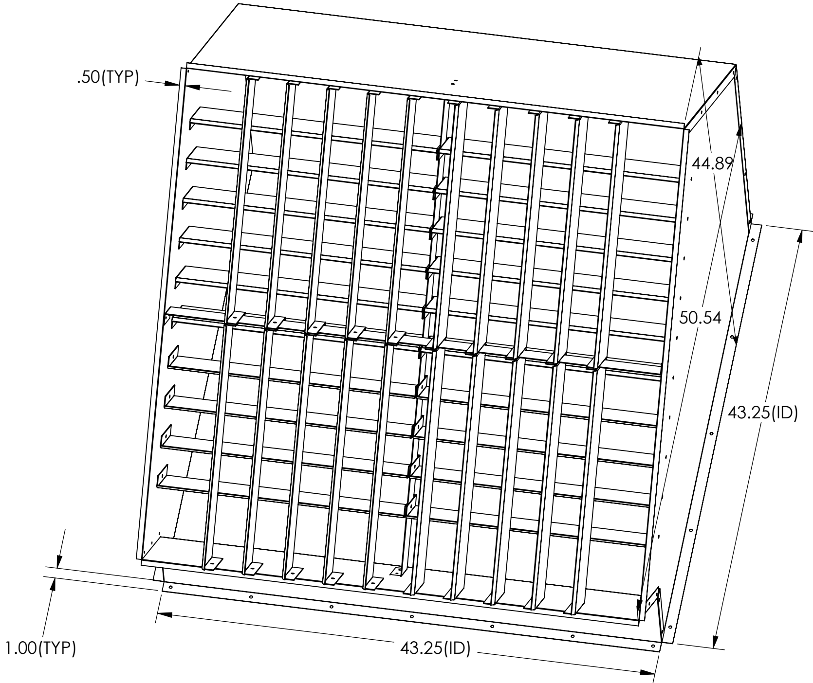
36 inch blower 45 degree
